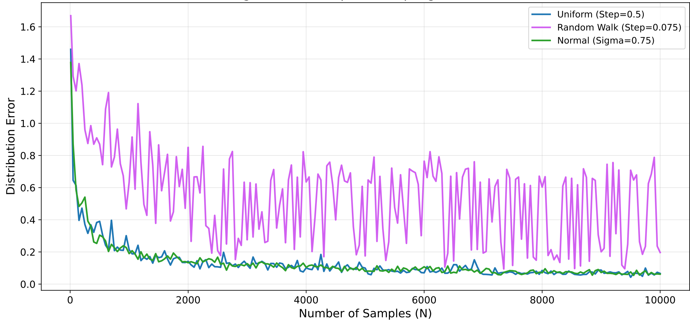
Convergence of Metropolis Sampling as N Increases
